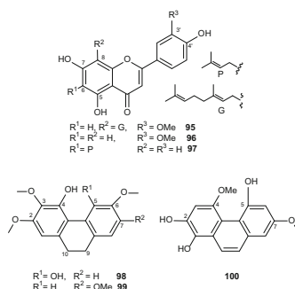
Fig. 17 Structures of non-cannabinoids 95–100
