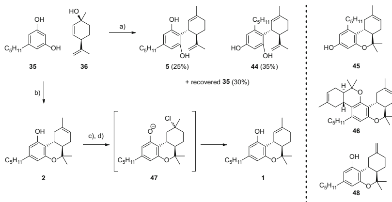
Scheme 6 Total synthesis of cannabidiol and (-)- \Delta^9 -trans-tetrahydrocannabinol ( 1 ) by Petrzilka and co-workers. Reagents and conditions: (a) 1.3 equiv N,N -dimethyl formamide-dineopentylacetal, CH 2 Cl 2 , rt, 63 h, 5 (25%), 34 (35%), and 32 (30%); (b) 0.15 equiv. p -TsOH, C 6 H 6 , reflux, 2 h, 2 (53%), 36 (13%), 37 (5%); (c) 0.67 equiv ZnCl 2 , HCl, CH 2 Cl 2 , 0°C to rt, 15 h, quantitative; (d) 3.2 equiv. K- t -amylate, C 6 H 6 , 5–65°C, 15 min, quantitative
