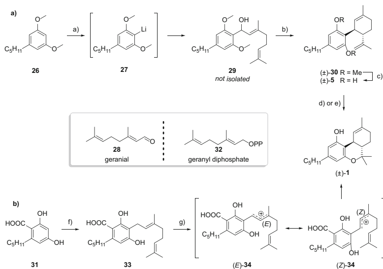
Scheme 4 First synthesis of racemic trans - \Delta^9 -tetrahydrocannabinol by Mechoulam and co-workers ( top ). Reagents and conditions: (a) 1.0 equiv n -BuLi, diethyl ether, rt, 2 h; then 1.0 equiv 28 , diethyl ether, rt; (b) 3.5 equiv p -TsCl, pyridine, rt, 3 d, 7% over two steps; (c) excess MeMgI (neat), 155–165°C, 15 min, 80%; (d) 0.05% (v/v) HCl in ethanol, reflux, 2 h, 2%; (e) 0.5 equiv \text{BF}_3 \cdot \text{Et}_2\text{O} , \text{CH}_2\text{Cl}_2 , rt, 30 min, 70%; (f) biosynthesis of (–)- trans - \Delta^9 -tetrahydrocannabinol ( bottom ). Reagents and conditions: (g) geranyl diphosphate 32 , olivetol geranyltransferase; (h) FAD, tetrahydrocannabinolic acid synthase (THCA) [39]
