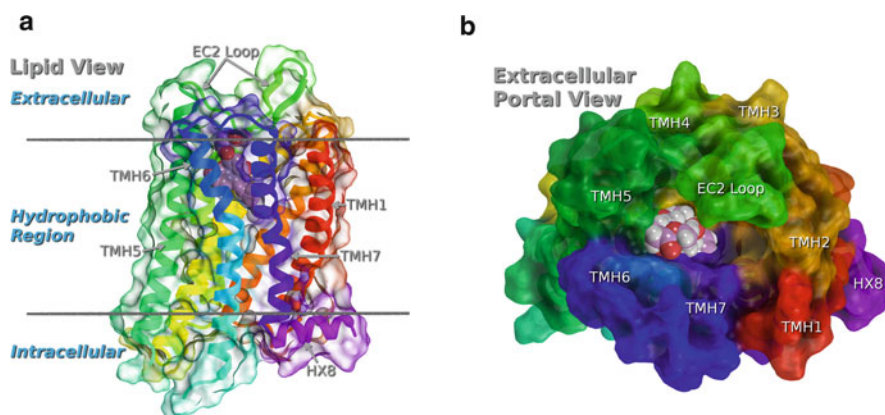
Fig. 3 (a) The typical Class A G-protein coupled receptor structure is illustrated by the 2.8 Å structure of the \mu opioid receptor (MOR; PDB entry 4DKL). (b) An extracellular view of the MOR structure is illustrated. In the MOR, the extracellular loops of the receptor are splayed open, making ligand access from the extracellular milieu possible. Here, the covalent ligand, beta-funaltrexamine is bound
