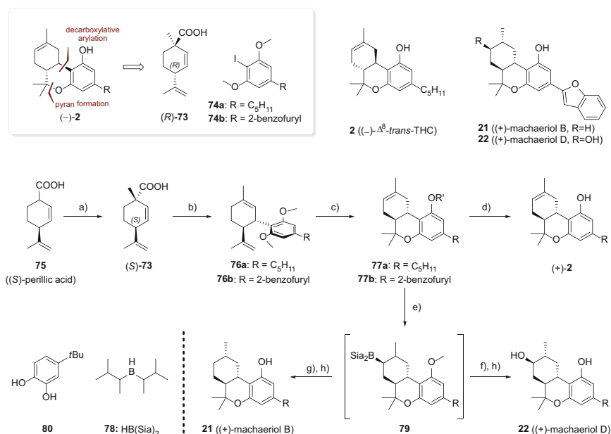
Scheme 9 Total synthesis of (+)- \Delta^8 -trans-tetrahydrocannabinol ((+)- 2 ) and machaeriols B ( 21 ) and D ( 22 ) by Studer and co-workers. Reagents and conditions: (a) 2.5 equiv LDA, THF, -78^\circ\text{C} to rt, 2 h; then 10 equiv DMPU, rt, 15 min; then 1.3 equiv dimethyl sulfate, -78^\circ\text{C} to rt, 1 h, 90% ( anti:syn 1.7:1); (b) 1.0 equiv 74a or 74b , 1.1 equiv Cs 2 CO 3 , 10 mol% Pd(dba) 2 toluene, reflux, 26 h, 74% for 76a , 81% for 76b ; (c) 2.0 equiv NaI, 1.5 equiv TMSI, acetonitrile, reflux, 24 h; then 0.2 equiv NaI, reflux, 24 h; (d) 10 equiv NaSEt, DMF, 140^\circ\text{C} , 12 h, 64% over two steps; (e) 4.0 equiv 78 , DCE, 60^\circ\text{C} , 2d; then (f) 4.9 equiv H 2 O, 6.6 equiv NaOH, 22 equiv H 2 O 2 , 0^\circ\text{C} to rt, 2 h, 51% over two steps or (g) 10 equiv 80 , reflux, 4 h; (h) 10 equiv NaSEt, DMF, 140^\circ\text{C} , 12 h, for 21 39% over 3 steps, for 22 82%
