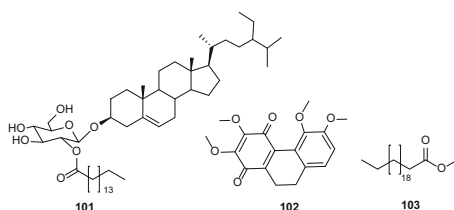
Fig. 18 Structures of non-cannabinoids 101–103
