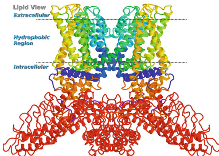
Fig. 10 The 3.27 Å structure of the TRPV1 channel
