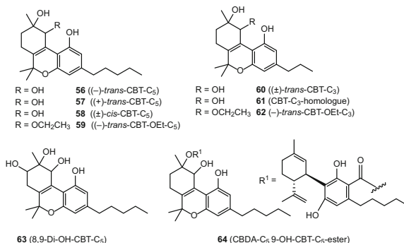
Fig. 11 Structures of cannabitrinol (CBT) type cannabinoids
