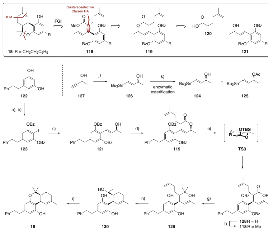
Scheme 15 Total synthesis of (–)-perrottetinene ( 18 ) by Kim and co-workers. Reagents and conditions: (a) 1.1 equiv I 2 , 1.1 equiv NaHCO 3 , THF/H 2 O, 0°C to rt, 10 min, 85%; (b) 2.2 equiv NaH, 2.2 equiv benzoyl chloride, 0°C to rt, 3 h, 98%; (c) 1.2 equiv 124 , 5 mol% Pd 2 (dba) 3 , 10 mol % P( t -Bu) 3 , 10 mol% CuI, 2.2 equiv CsF, toluene, 80°C, 5 h, 78%; (d) 1.5 equiv 120 , 1.5 equiv DCC, 30 mol% DMAP, CH 2 Cl 2 , 0°C to rt, 16 h, 98%; (e) 2.0 equiv TBSCl, 2.0 equiv LDA, THF/HMPA (4:1), –78°C to rt, 15 h, 60%; (f) 1.5 equiv DCC, 30 mol% DMAP, CH 2 Cl 2 /MeOH, rt, 16 h, 91%; (g) 29 equiv MeMgBr, THF, reflux, 2 h, 90%; (h) 5 mol% Grubbs second generation catalyst, CH 2 Cl 2 , reflux, 16 h, 90%; (i) 2.3 mol% p -TsOH, C 6 H 6 , reflux, 30 min, 55%; (j) 1.3 equiv Bu 3 SnH, 1 mol% Pd(PPh 3 ) 2 Cl 2 , THF, –78°C, 2 h, 81%; (k) lipozyme, diisopropyl ether/vinyl acetate (10:1), 35°C, 12 h, 47% ( 124 , >99% ee ) and 48% ( 125 , >99% ee )
