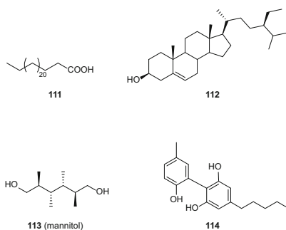
Fig. 21 Structures of non-cannabinoids 111–114
