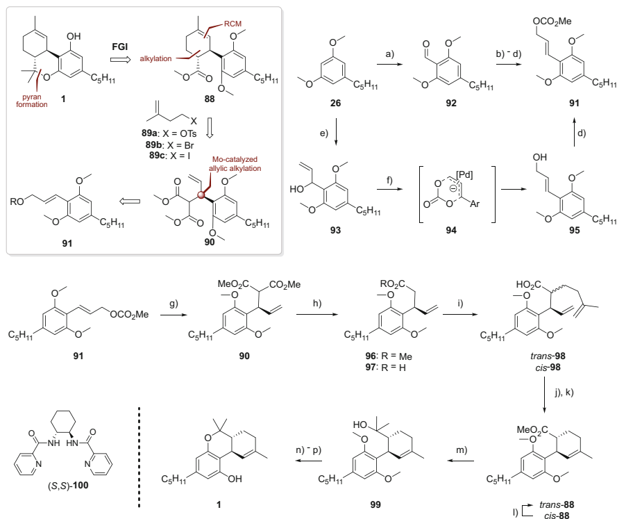
Scheme 11 Asymmetric synthesis of 1 as reported by Trost and co-workers. Reagents and conditions: (a) 1.1 equiv n -BuLi, THF, reflux, 2.5 h; then 1.1 equiv dimethyl formamide, rt to reflux, 3 h, 83%; (b) 1.1 equiv NaH, 1.1 equiv triethylphosphonoacetate, THF, -35^{\circ}\text{C} to rt, 1 h; (c) 2.5 equiv DIBAL, diethyl ether, -10^{\circ}\text{C} to 0^{\circ}\text{C} , 30 min, 97%; (d) 1.1 equiv n -BuLi, 2.0 equiv methyl chloroformate, diethyl ether, -78^{\circ}\text{C} , 10 min, quantitative; (e) 1.1 equiv n -BuLi, THF, -78^{\circ}\text{C} to rt, 2 h, 91%; (f) n -BuLi, \text{CO}_2 , cat. \text{PdCl}_2(\text{CH}_3\text{CN})_2 ; (g) 1.2 equiv dimethyl malonate, 1.2 equiv NaH, 10 mol% \text{Mo}(\text{CO})_3(\text{C}_7\text{H}_8) , 15 mol% ( S,S )- 100 , THF, 75^{\circ}\text{C} , 54 h, 84% (97% ee ); (h) 1 N aq. NaOH, MeOH, reflux, 6 h; then 160^{\circ}\text{C} , 1 h, 98%; (i) 2.4 equiv LDA, THF, -20^{\circ}\text{C} to 40^{\circ}\text{C} , 30 min; then 1.5 equiv 89c , -10^{\circ}\text{C} to rt, 3 h, 84% ( trans/cis 2.4:1); (j) 3.0 equiv \text{K}_2\text{CO}_3 , 3.0 equiv dimethyl sulfate, acetone, reflux, 3 h; (k) 1 mol% Grubbs second generation catalyst, \text{CH}_2\text{Cl}_2 , rt, overnight; then 0.5 mol% Grubbs second generation catalyst, \text{CH}_2\text{Cl}_2 , rt, 16 h, 93%; (l) 1 M NaOMe, MeOH, reflux, 3 d, 92% ( trans/cis 1:0.03); (m) 3.0 equiv MeLi, diethyl ether, -78^{\circ}\text{C} to rt, 92%; (n) 3.0 equiv NaSEt, DMF, 140^{\circ}\text{C} , 3 h, 97%; (o) 2.0 equiv \text{ZnBr}_2 , \text{MgSO}_4 , \text{CH}_2\text{Cl}_2 , rt, overnight; (p) 10.0 equiv NaSEt, DMF, 140^{\circ}\text{C} , 10 h, 61% over two steps
