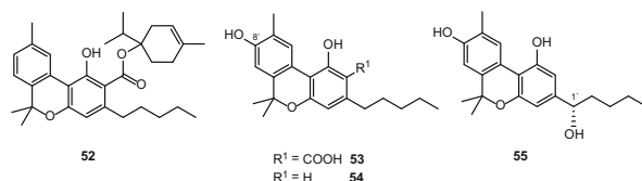
Fig. 10 Structures of cannabinol (CBN) type cannabinoids
