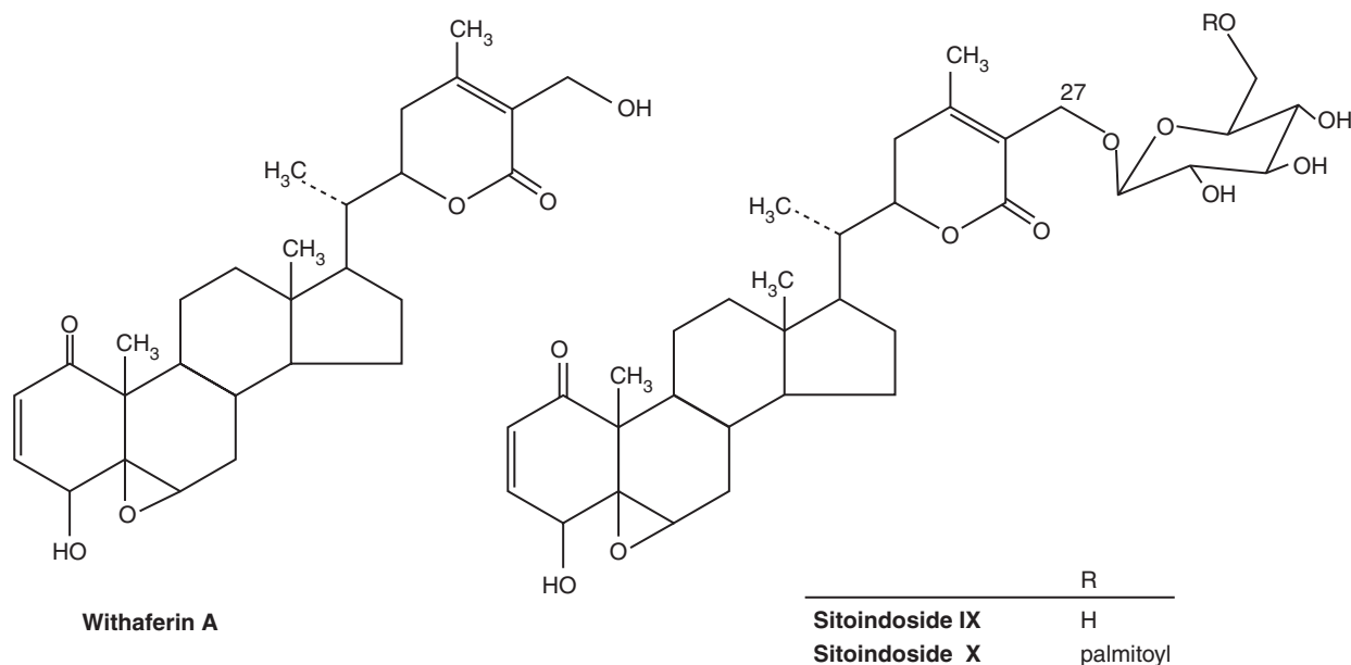
Withanolides
