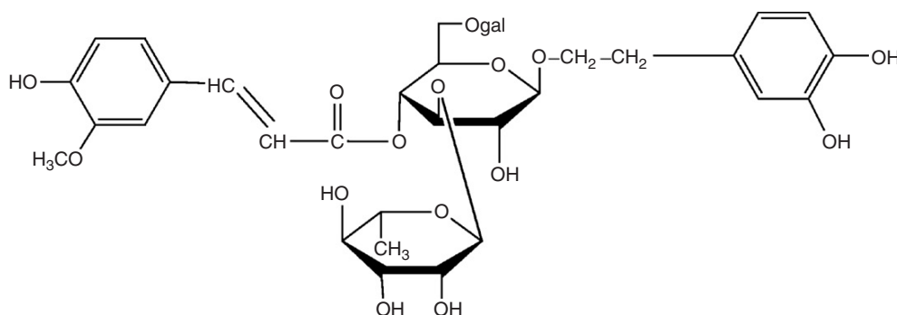
Jioglutoside A
