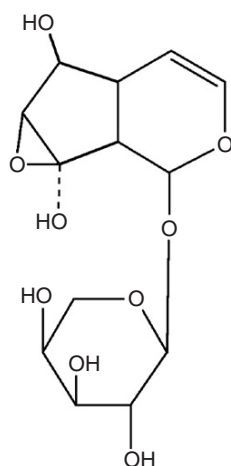
Jioglutoside A
