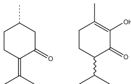
(–)-Pulegone
