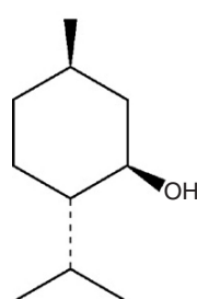
(–)-Menthol
