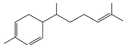
Zingiberene
