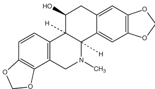
Chelidonine
