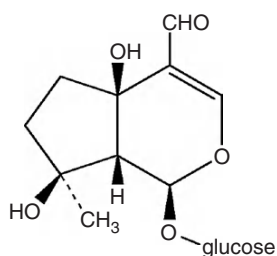
Euphroside
