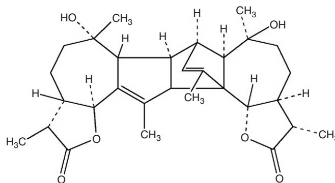
Absinthin
