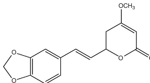
Methysticin
