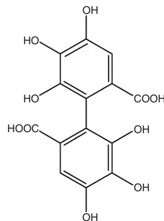
Hexahydroxydiphenic acid
