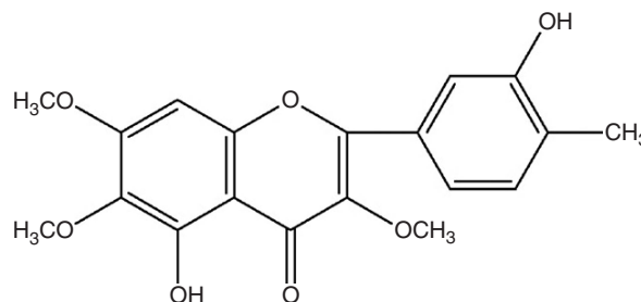
Casticin
