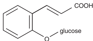
Melilotoside
