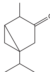
Thujone
