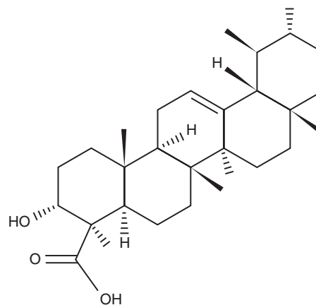
beta-Boswellic acid
