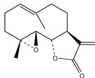
Parthenolide
