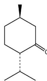
(–)-Menthone
