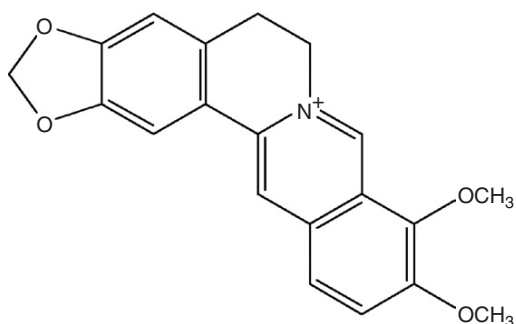
Berberine
