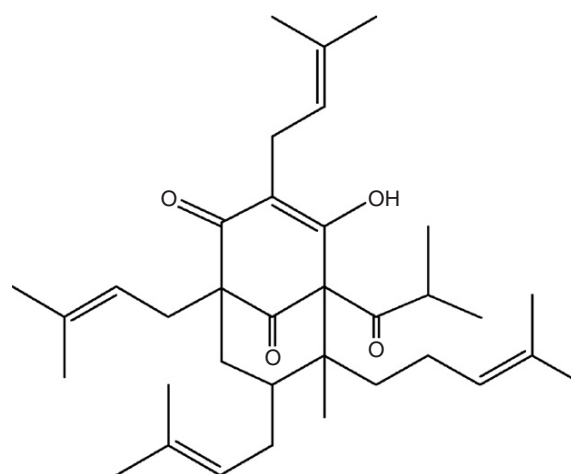
Hyperforin
