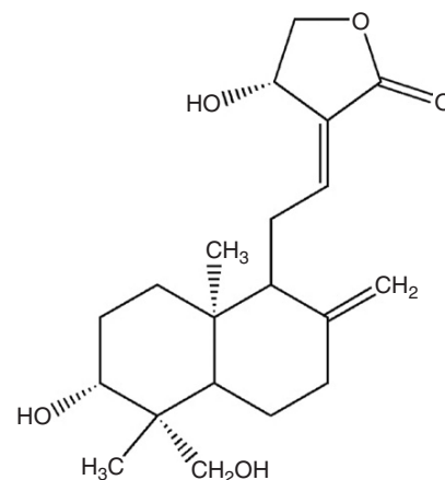
Andrographolide
