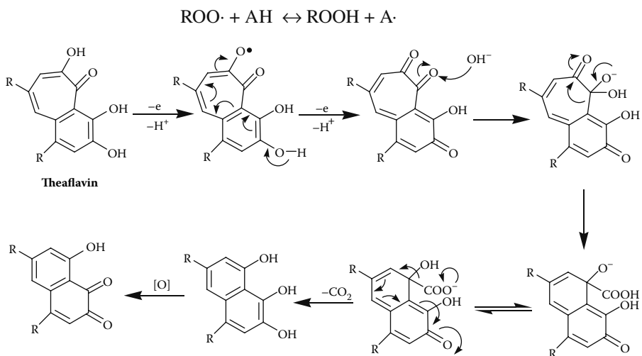
FIGURE 8.14 Proposed scavenging mechanism of theaflavin to 2,2-diphenyl-1-picrylhydrazyl and hydrogen peroxide. (From Jhoo, J., Lo, C., Li, S., Sang, S., Ang, C. Y. W., Heinze, T. M., and Ho, C.-T. 2005. Stability of black tea polyphenol, theaflavin, and identification of theanaphthoquinone as its major radical reaction product. J. Agric. Food Chem. 53:6146–50. With permission.)
