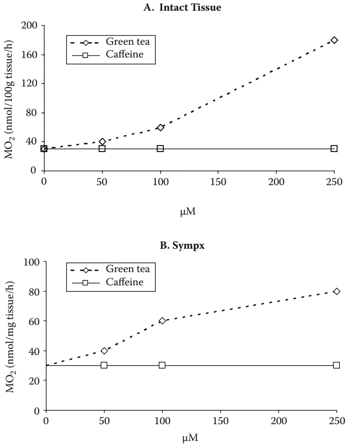
FIGURE 13.2 Respiration rates ( \text{MO}_2 ) of interscapular brown adipose tissue (IBAT) from intact rats (A) and from rats chemically sympathectomized (B) in response to caffeine or to green tea extract containing isomolar concentrations of caffeine. (Modified from Dulloo, A. G., Seydoux, J., Girardier, L., Chantre, P., and Vandermander, J. 2000. Green tea and thermogenesis: Interactions between catechin-polyphenols, caffeine and sympathetic activity. Int. J. Obesity 24:252–58.)
