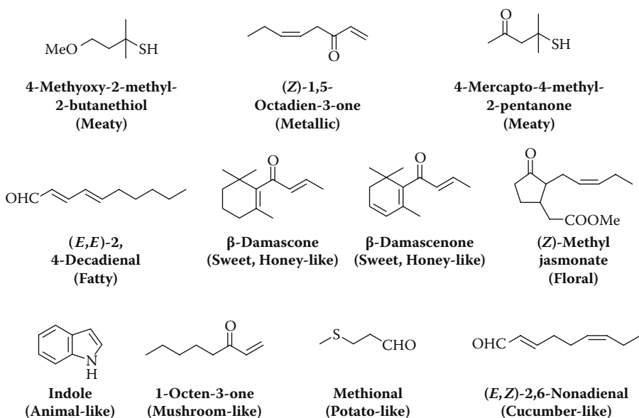
FIGURE 17.7 Potent flavor components of green tea drink identified by AEDA. Nonretorting process. FD factor of the flavor components: greater than 500.
