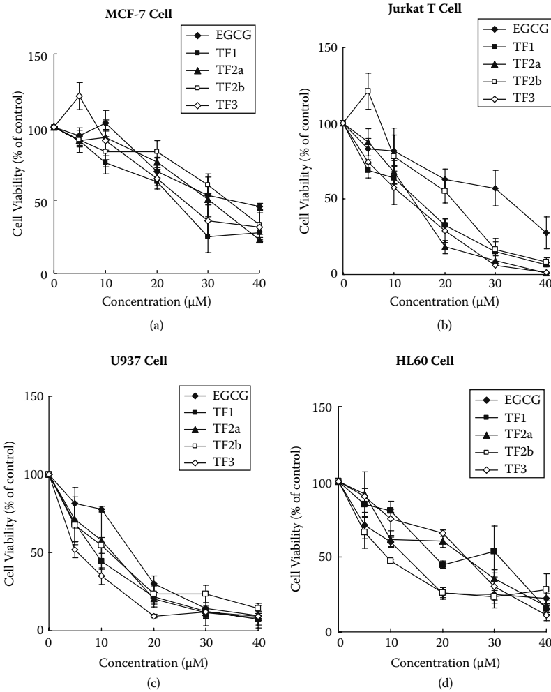
FIGURE 11.2 The effect of the tea polyphenols on the viability of different cell lines. 1 \times 10^4 cells were seeded in 96-well plates and treated with various doses of tea polyphenols. After 24 h incubation, cell viability was determined by ATPLite-M cytotoxicity assay. Results were obtained from three independent experiments as mean \pm SD.
