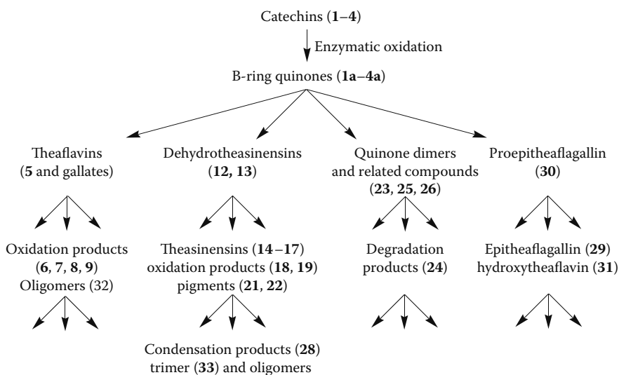
FIGURE 5.9 Catechin oxidation cascade.
