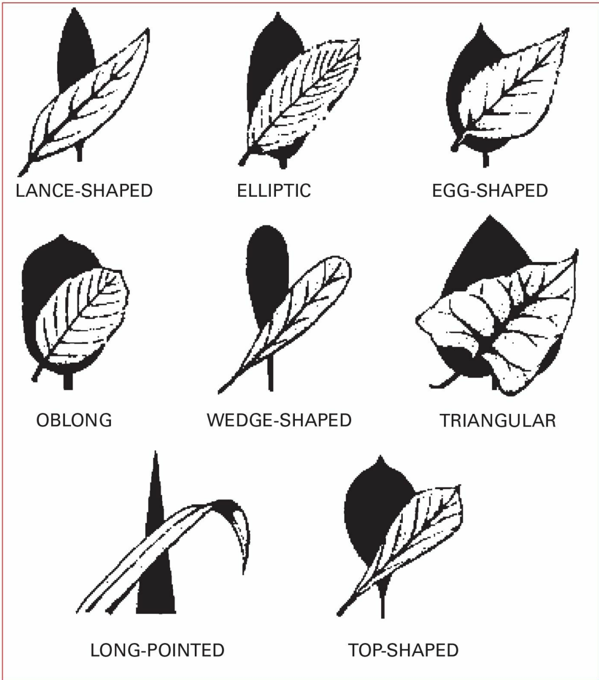
Figure 1.2 Leaf shapes.
