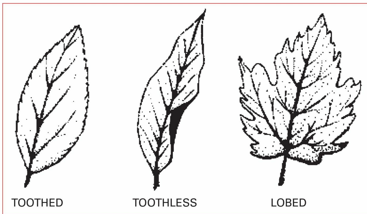
Figure 1.1 Leaf margins.
