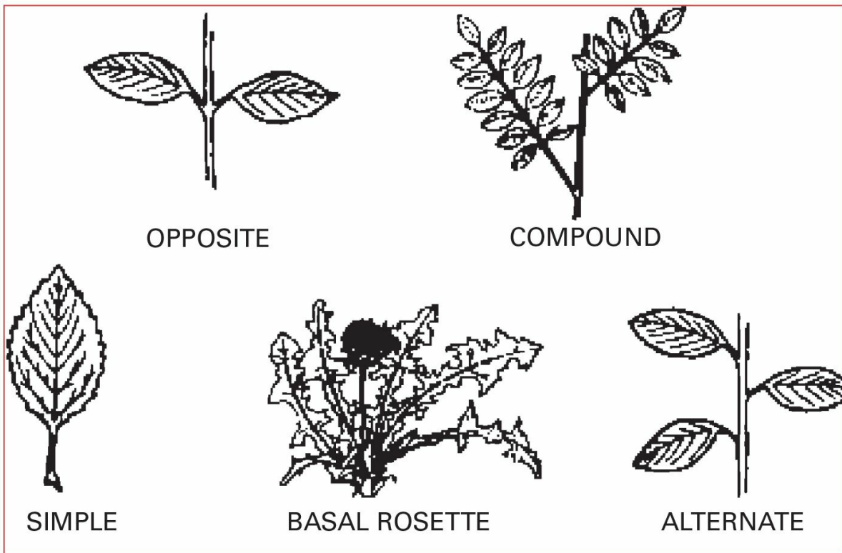
Figure 1.3 Leaf arrangements.
