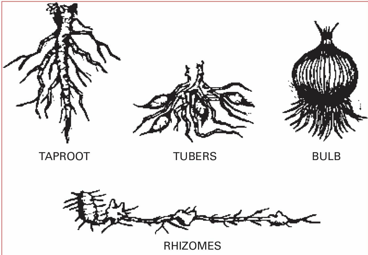
Figure 1.4 Root structures.
