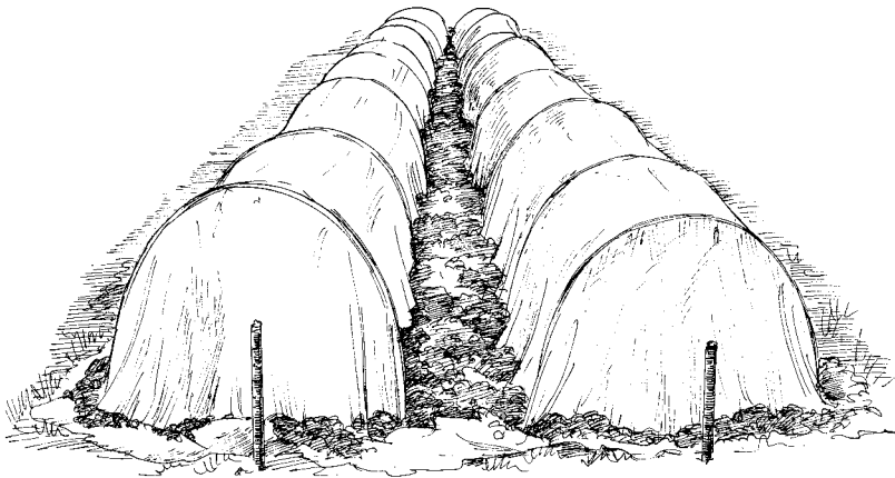
Low tunnels made with ½" galvanized electrical wire conduit and row cover
