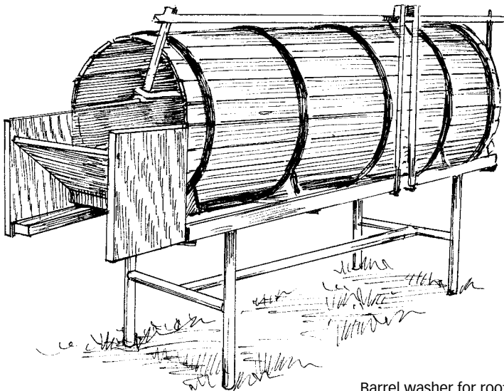
Barrel washer for root vegetables
