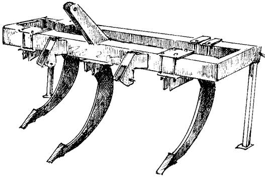
Three-shank subsoiler
