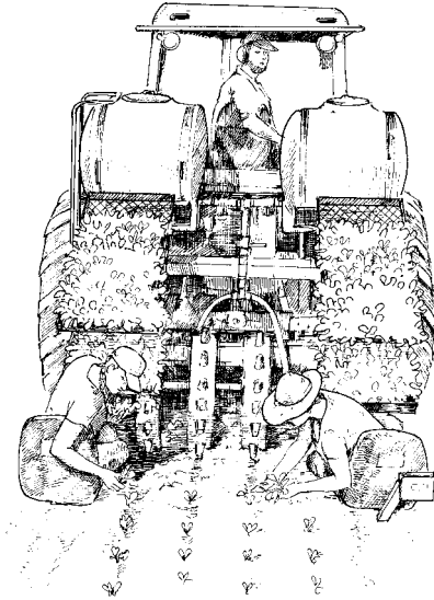
Transplanting four rows of lettuces with a waterwheel transplanter
