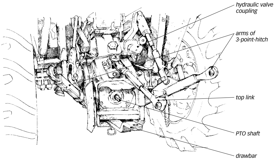
Rear view of tractor
