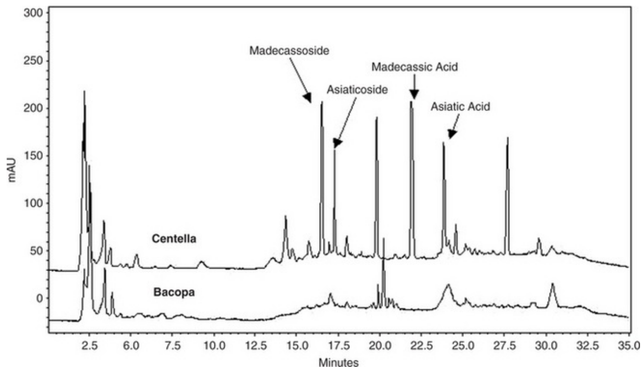
Fig. 1-2 HPLC trace of Bacopa ( Bacopa monnieri ) and gotu kola ( Centella asiatica ) extracts showing the peaks of the major active constituents in gotu kola.
