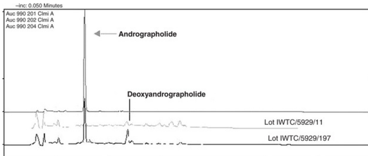
Fig. 1-5 HPLC trace showing key marker compounds present and absent in two herbal extracts of Andrographis paniculata .
