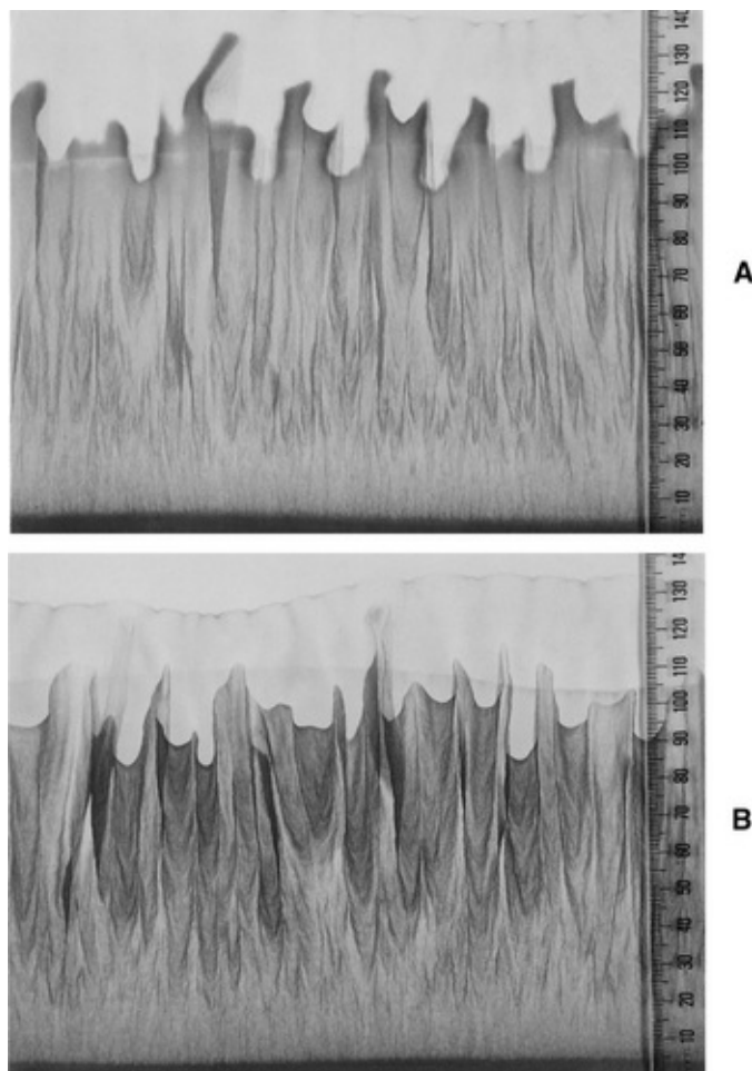
Fig. 1-1 A visual comparison of a dried plant extract ( A ) and fresh plant tincture ( B ) obtained by a paper chromatography technique (vertical capillary dynamolysis).
