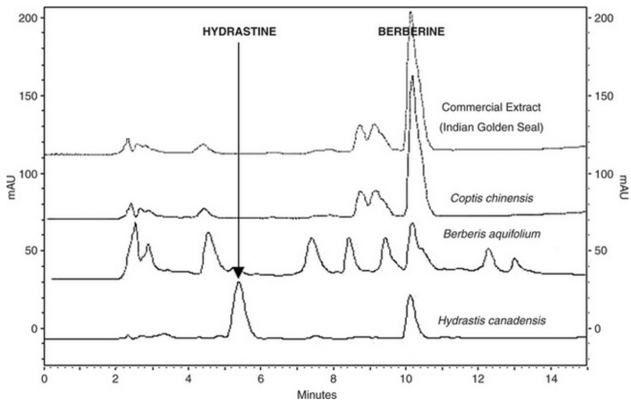
Fig. 1-3 HPLC trace of golden seal, golden thread, Oregon grape, and an adulterated commercial herbal extract. The constituent hydrastine is contained only in the authentic golden seal extract.
