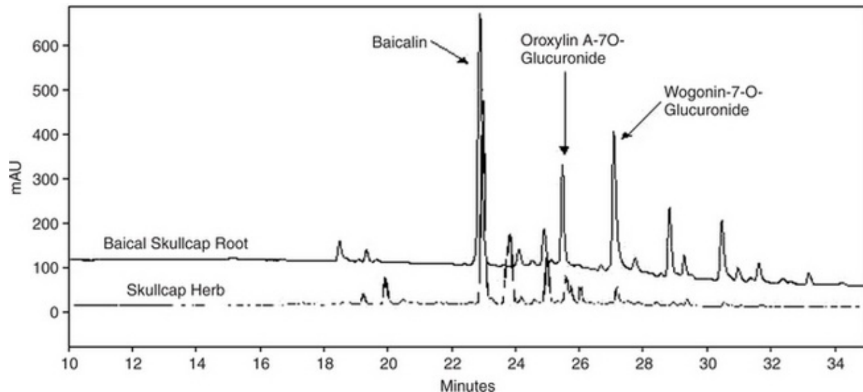
Fig. 1-4 HPLC trace of skullcap and Baical skullcap showing the main flavonoids present in each herbal extract.
