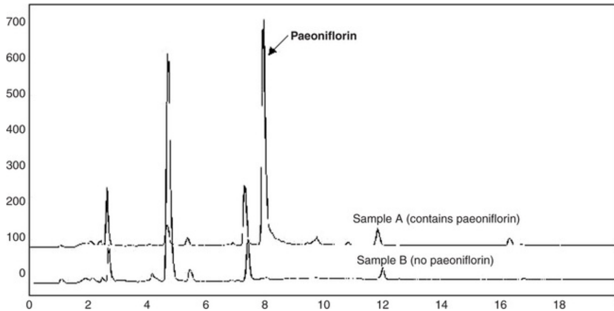
Fig. 1-6 HPLC trace of two white peony ( Paeonia lactiflora ) extracts indicating the presence or absence of the marker compound paeoniflorin.
