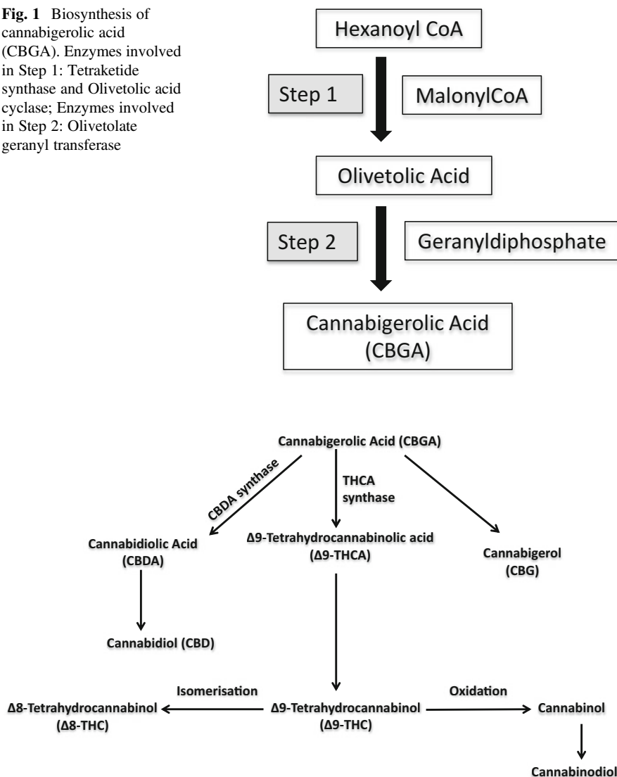
Fig. 2 Biosynthesis of important phytocannabinoids
